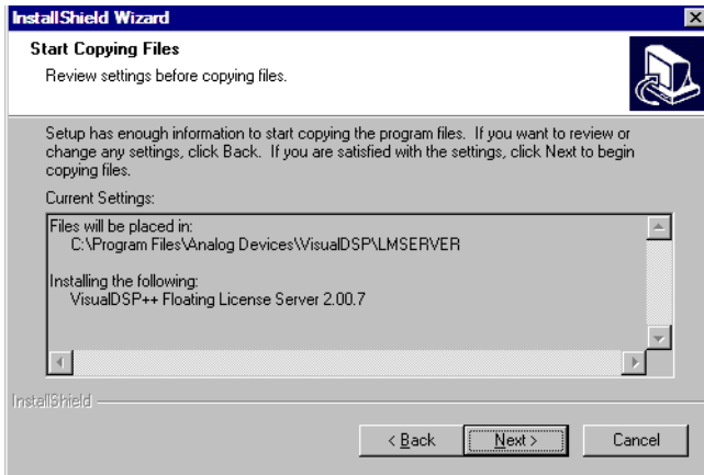
Figure 3-1. InstallShield Wizard
